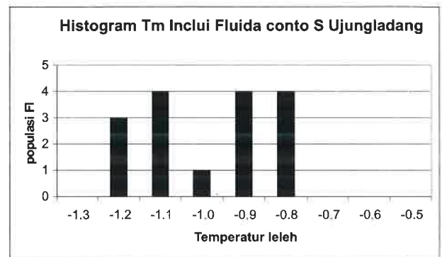
Gambar 3 Histogram Tm Includi Fluida Conto S
